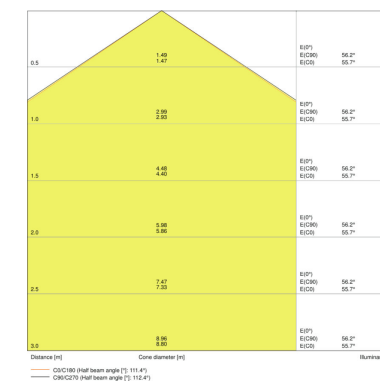
DP 5TH 1500 46W 840 IP65 GY
